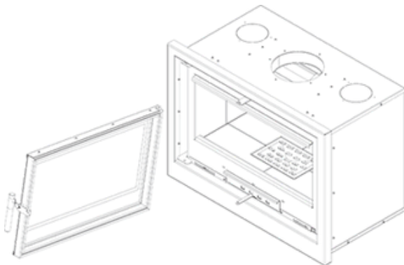
Fig. 12. ARKE cassette - dismantling the door, step 6
